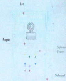
Fig. 1. paper chromatography
